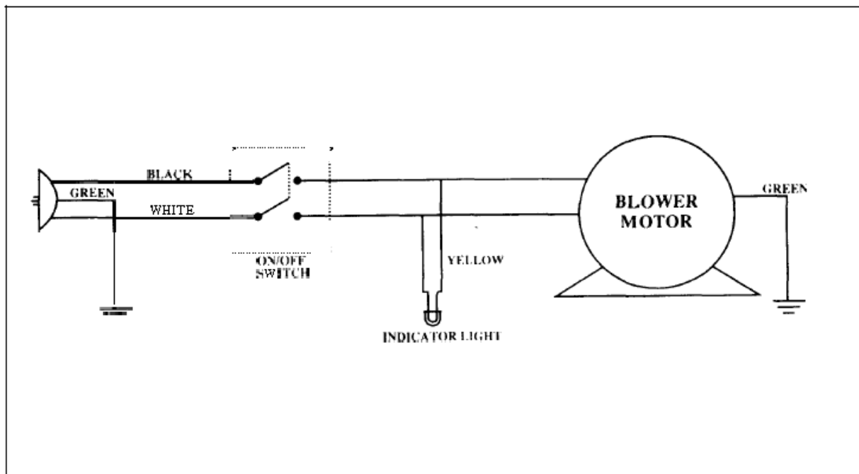
FIGURE 4 - ELECTRICAL SCHEMATIC
